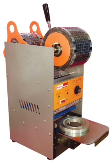
Semi Auto Cup Sealer (Lever)
